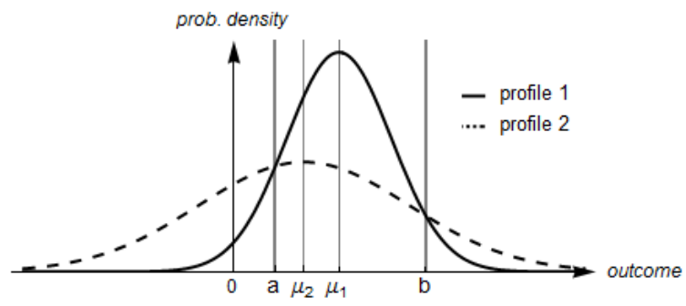
Figure 1: Probability density functions of two alternative behaviors.
