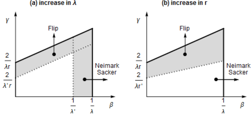
Figure 1: Qualitative sketch of the region of local asymptotic stability of the FSS in the plane of parameters \beta and \gamma , for given values of \lambda and r . Left panel: stability region for given \lambda and \lambda' ( \lambda' > \lambda ). Right panel: stability region for given r and r' ( r' > r ).
