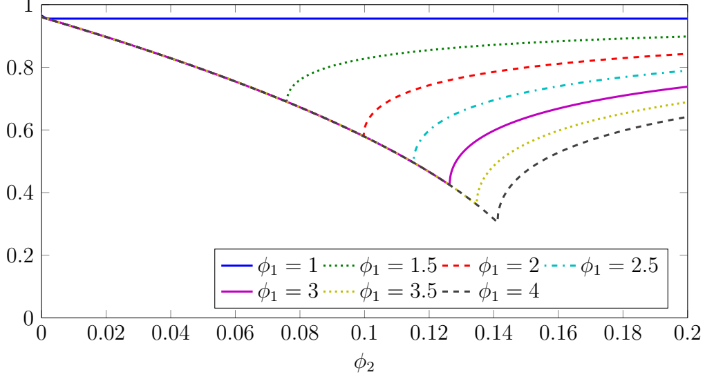
Figure 8: Absolute value of largest eigenvalue of LTL model as function of \phi_2 for different values of \phi_1 .
