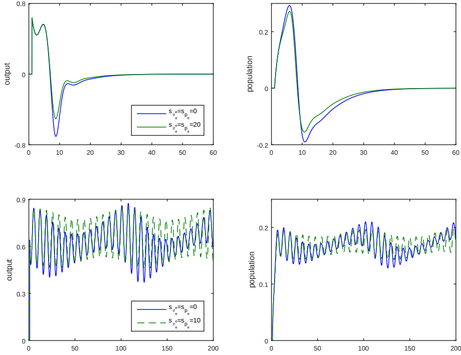
Figure 7: Dynamic adjustments of the full 4D model (Y, p_e, \pi_e^e, x) for different values of s_{p_e} and s_{\pi_e^e} for the dynamically stable case (upper panels) and the explosive case (lower panels).
