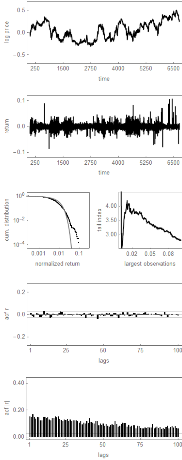
Figure 4: The dynamics of a small-scale model in which only fundamentalists obtain sunspots (S-0F model). The panels show from top to bottom the evolution of the log price, the returns, the cumulative distribution of normalized returns, the Hill tail index estimator as a function of the largest returns and the autocorrelation functions of raw and absolute returns, respectively.
